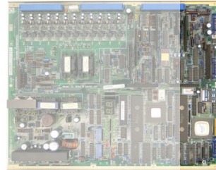
E4809-045-145-C or 1006-1107 Okuma VACIII Drive Board
